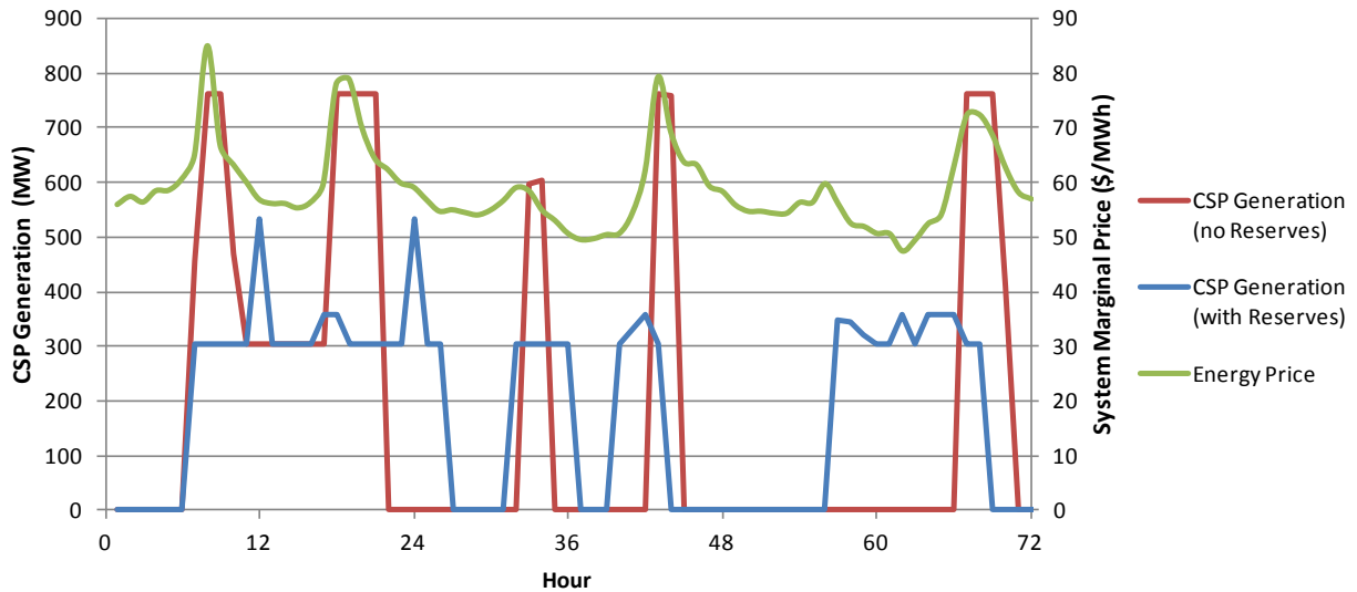
Figure 7. CSP operation for three days starting January 31 when providing only energy and providing both energy and reserves
