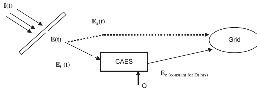
Fig. 2. The PV-CAES conceptual model.
