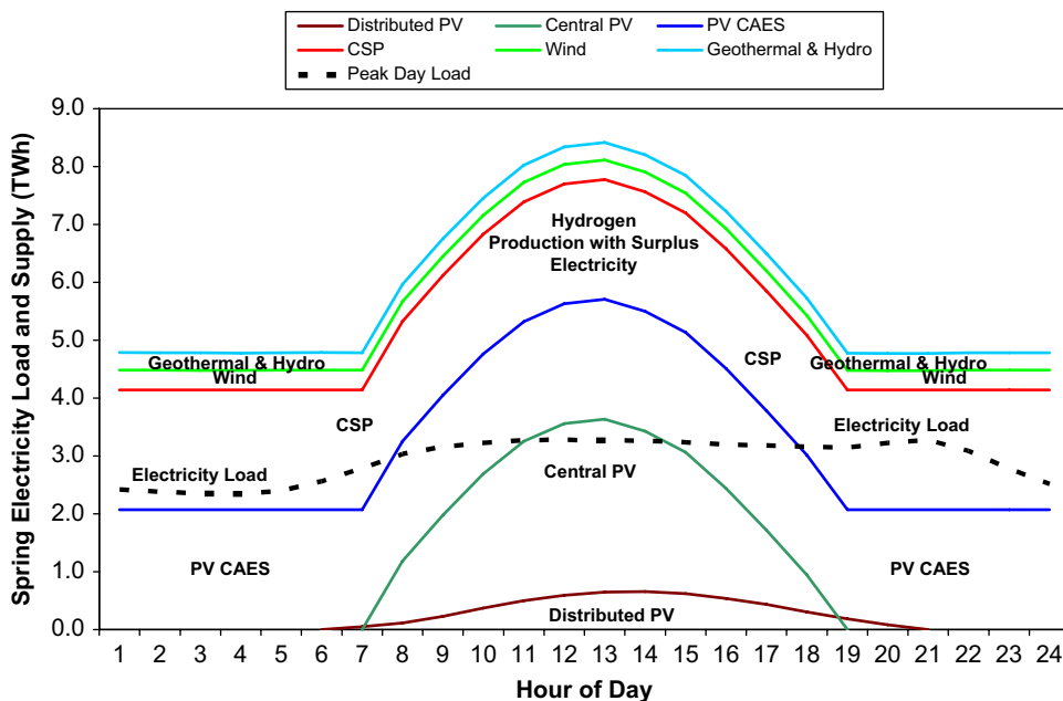
Fig. 10. 2100 spring electricity load and supply scenario.
