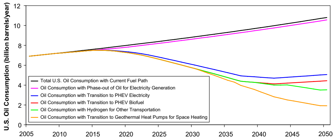
Fig. 7. US annual oil consumption with the current energy path and reductions corresponding to each of the technologies of the renewable energy path. (Each curve shows additional oil reduction; the bottom curve shows the total oil consumption in the renewable energy path.)
