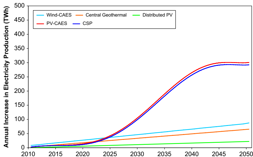
Fig. 6. Annual added electricity production from renewable energy.
